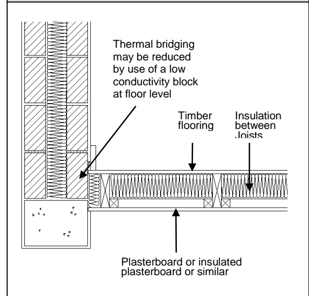
Diagram B18 Exposed timber floor, insulation between joists (Par. B.7.4)
