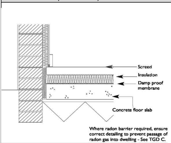
Diagram B13 Concrete slab on ground floor, insulation under screed (Par. B.7.1)
