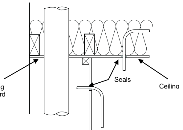
4. SEALING AROUND SERVICE PIPES
