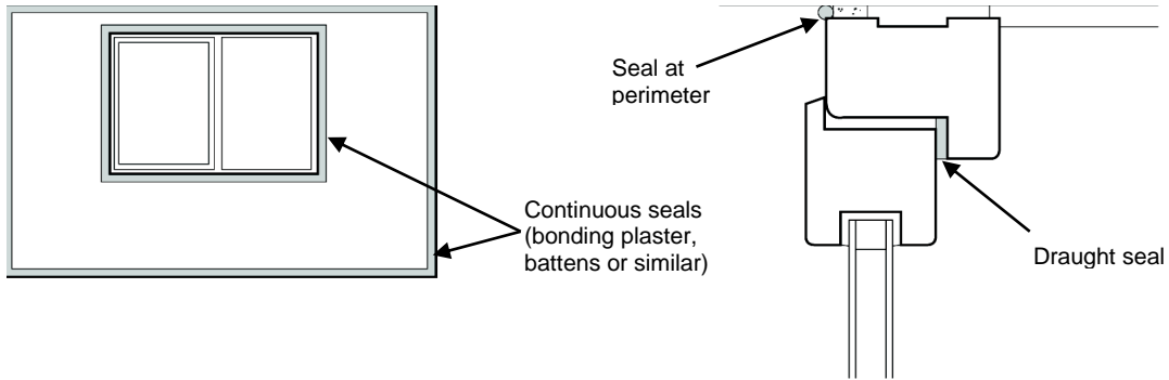
1. POSITION OF CONTINUOUS SEALING BANDS FOR DRY-LININGS FIXED TO MASONRY WALLS
