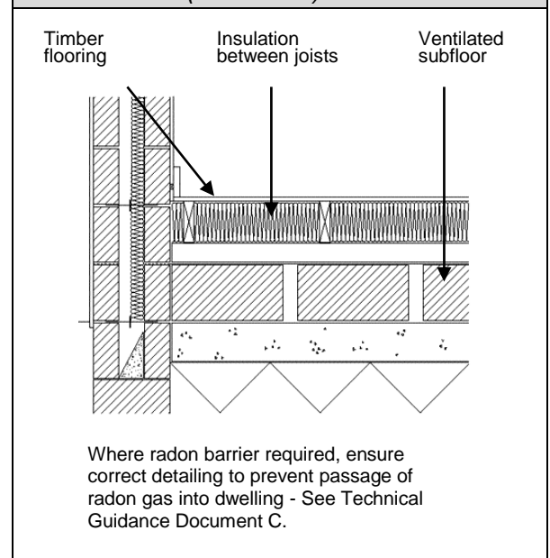
Diagram B14 Suspended timber floor with quilt insulation (Par. B.7.2)
